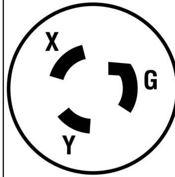
Plug
